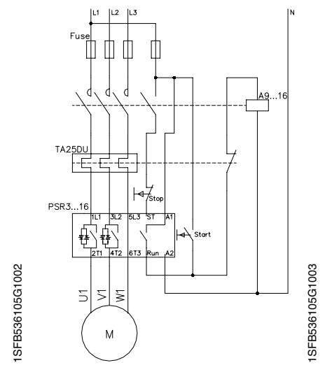
F) With fuses, contactor and O.L.
