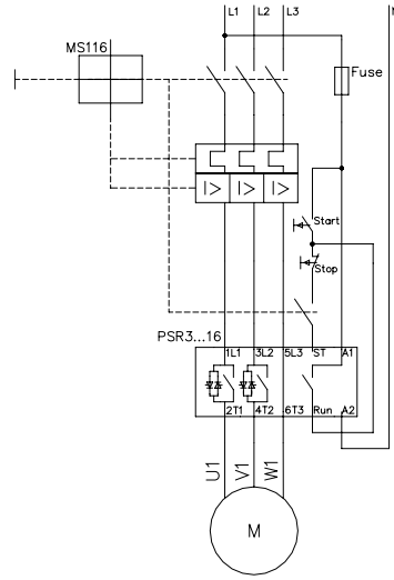
E) With MMS and auxiliary contact
