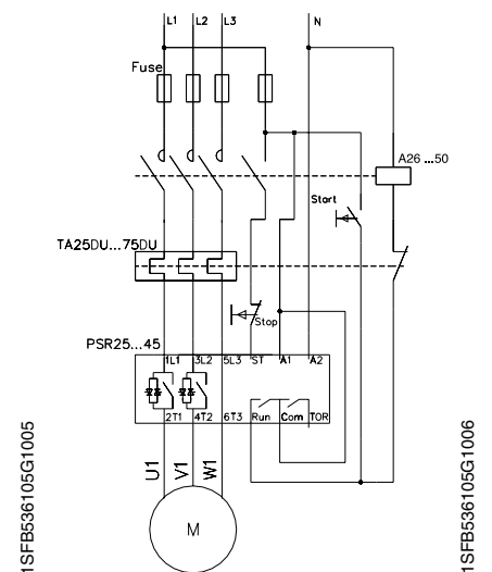
I) With fuses, contactor and O.L.
