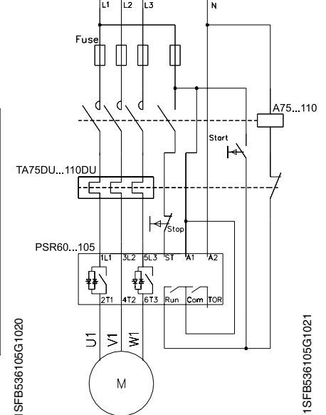
I) With fuses, contactor and O.L.
