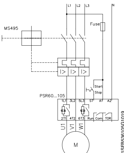
PSR60 ... 105 G) With MMS
