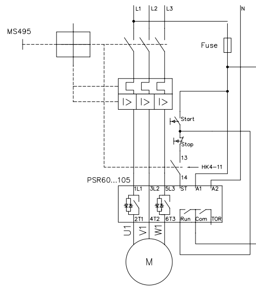
H) With MMS and auxiliary contact
