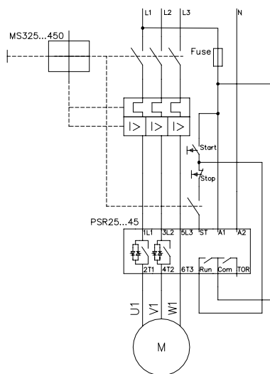
H) With MMS and auxiliary contact
